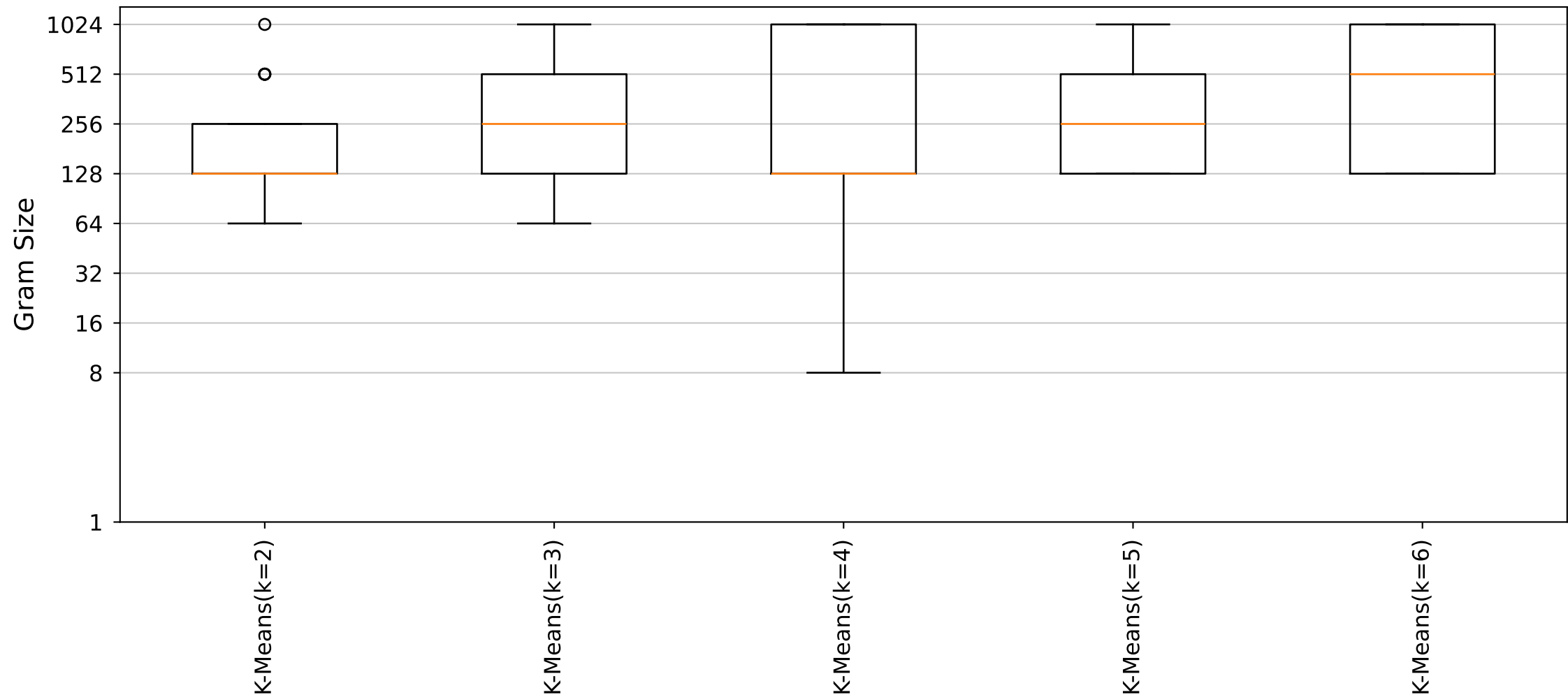
YARA Rules Gram Size Distribution (Cluster29_Size6 dataset)
